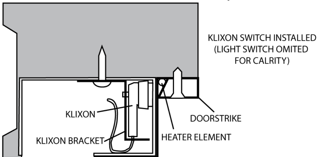
SECTION OF LIGHT SWITCH JUNCTION BOX
